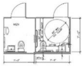
Two Stall with ADA Lavatory.
