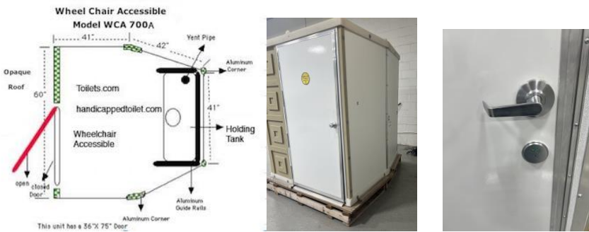
Fig. 7 Model 700A Handicapped Portable Toilet
