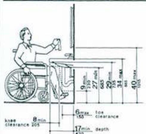
Fig. 31 Lavatory Clearances
