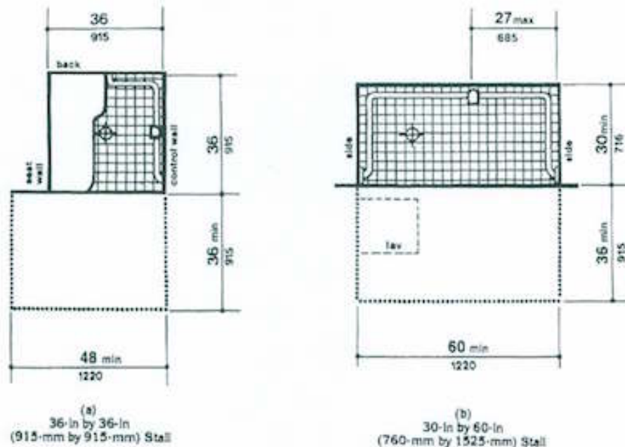
Fig. 35 Shower Size and Clearances
